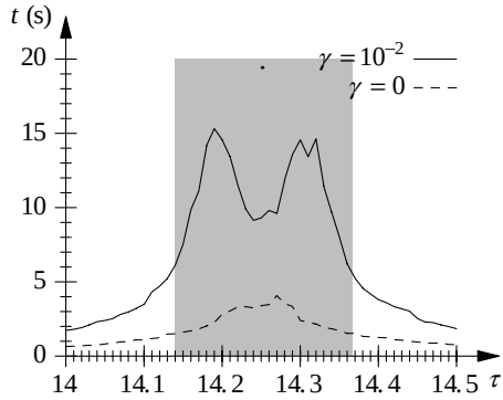
Fig. 3. Verification time
