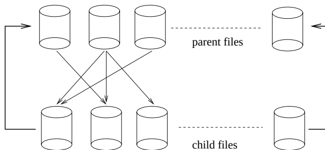
Fig. 1. Externally stored state space with parent and child files
