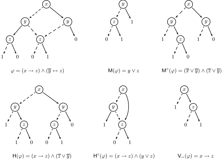
Fig. 3. ROBDDs for (x \rightarrow z) \wedge (\overline{y} \leftrightarrow z) and some approximations of it
