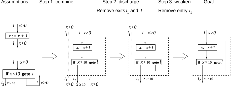
Fig. 4. An example to illustrate \mathcal{L}_c 's composition rules
