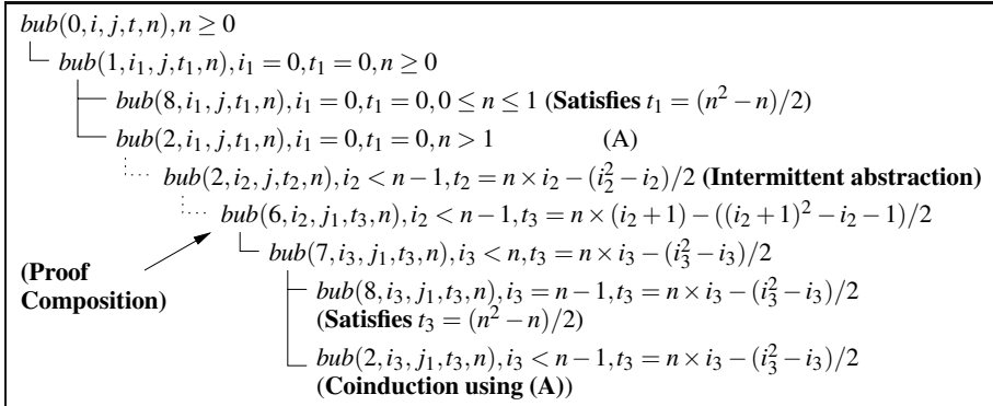
Fig. 6. Compositional Proof
