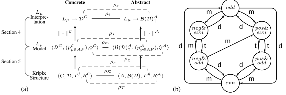
Fig. 2. (a) Abstraction L_\mu : the top row summarizes soundness relations for abstracting L_\mu interpretations; the middle one – L_\mu models, i.e., interpretations of atomic propositions and \diamond relation; the bottom one – L_\mu -preserving abstractions of Kripke structures. (b) A fragment of the abstraction \alpha_T(R_1) , where R_1(x) = x + 1 .
